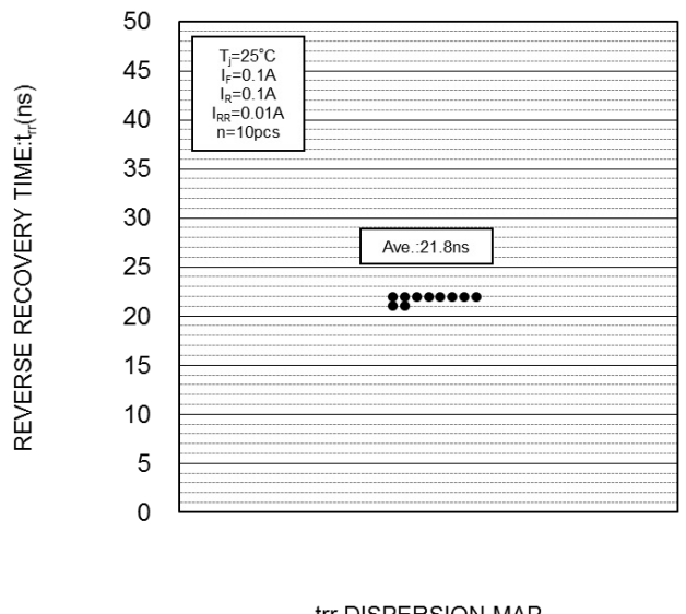
t_{rr} DISPERSION MAP
